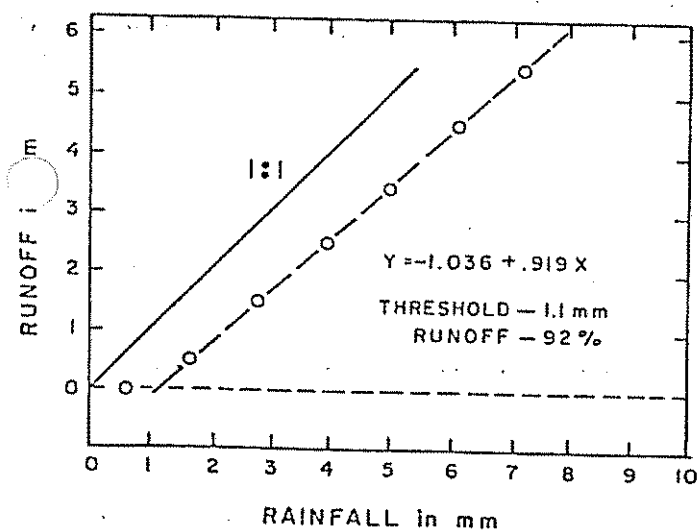
Fig. 2. Rainfall runoff relationship as determined with portable plot sprinkler.
